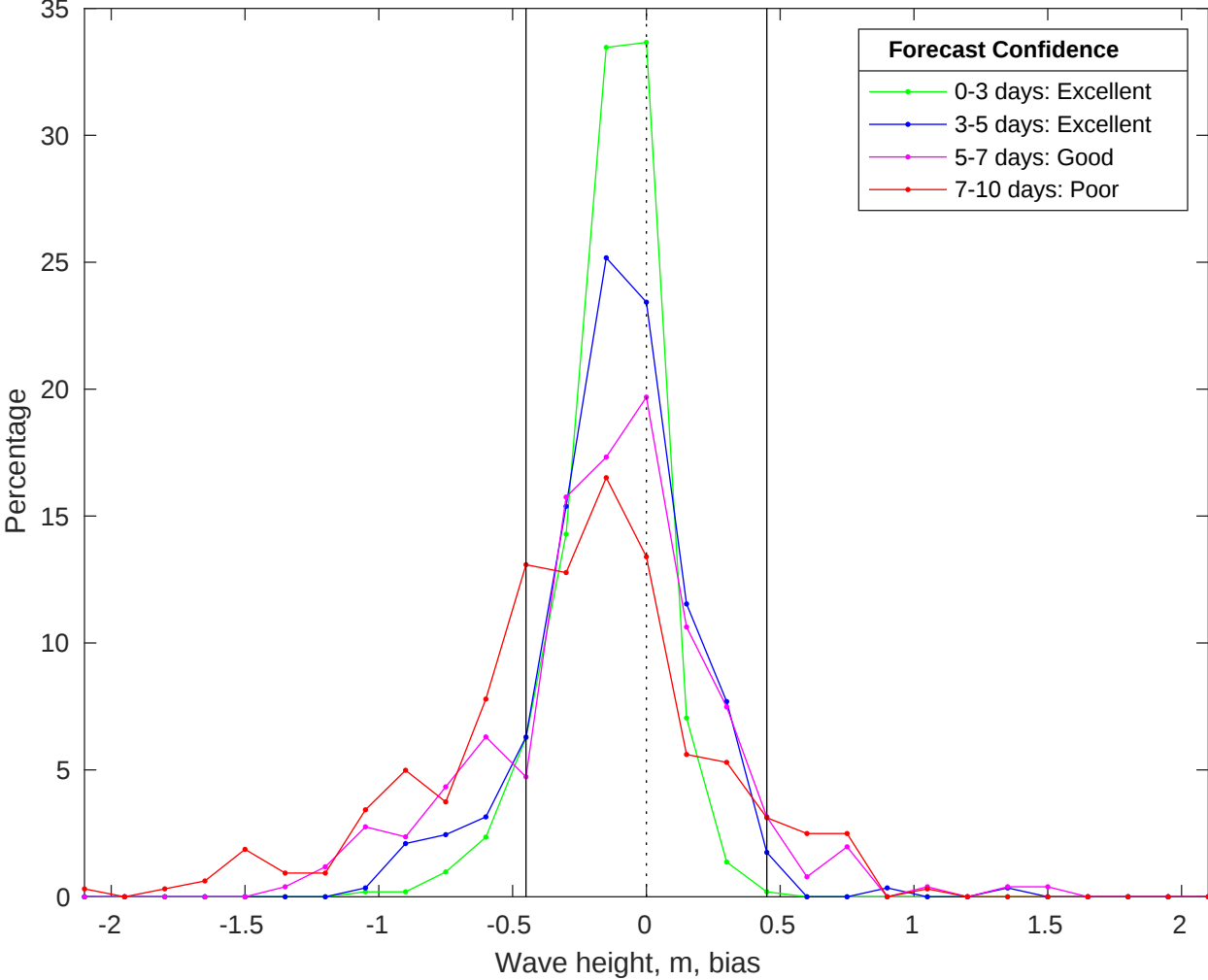
NDBC 41013 vs CMEMS Waves Bias Histogram: 22-Jan-2026
