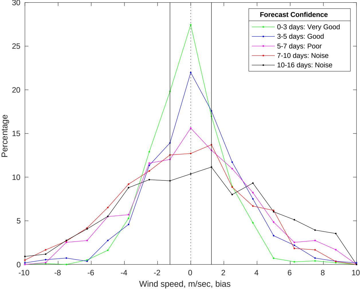
NDBC 41013 vs GFS Winds Bias Histogram: 22-Jan-2026
