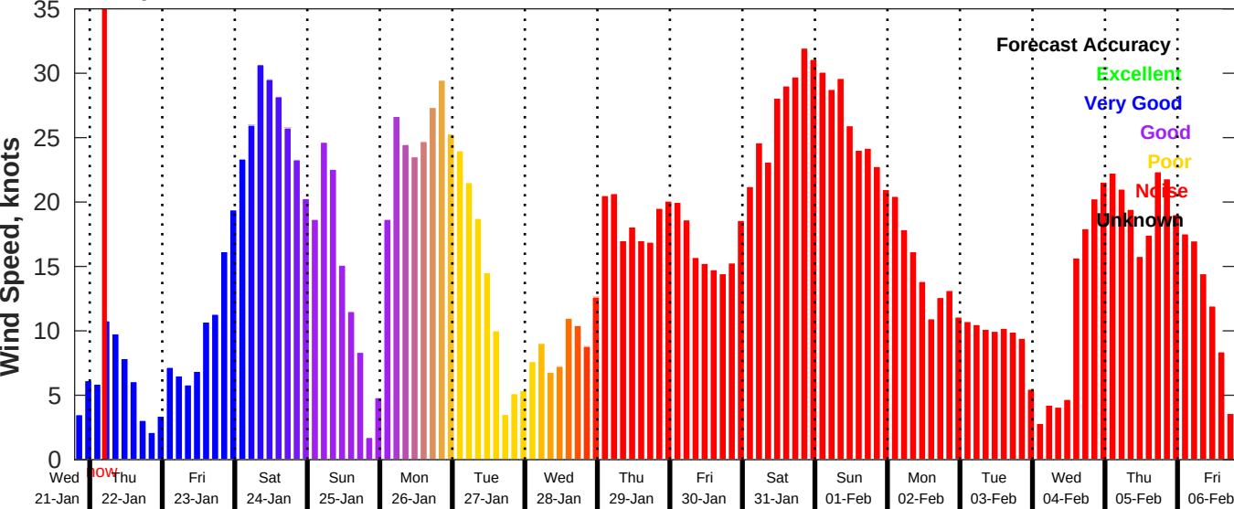
GFS Wind Speed Forecast for NDBC 41013 from 21-Jan-2026 19:00:00 to 06-Feb-2026 19:00:00
