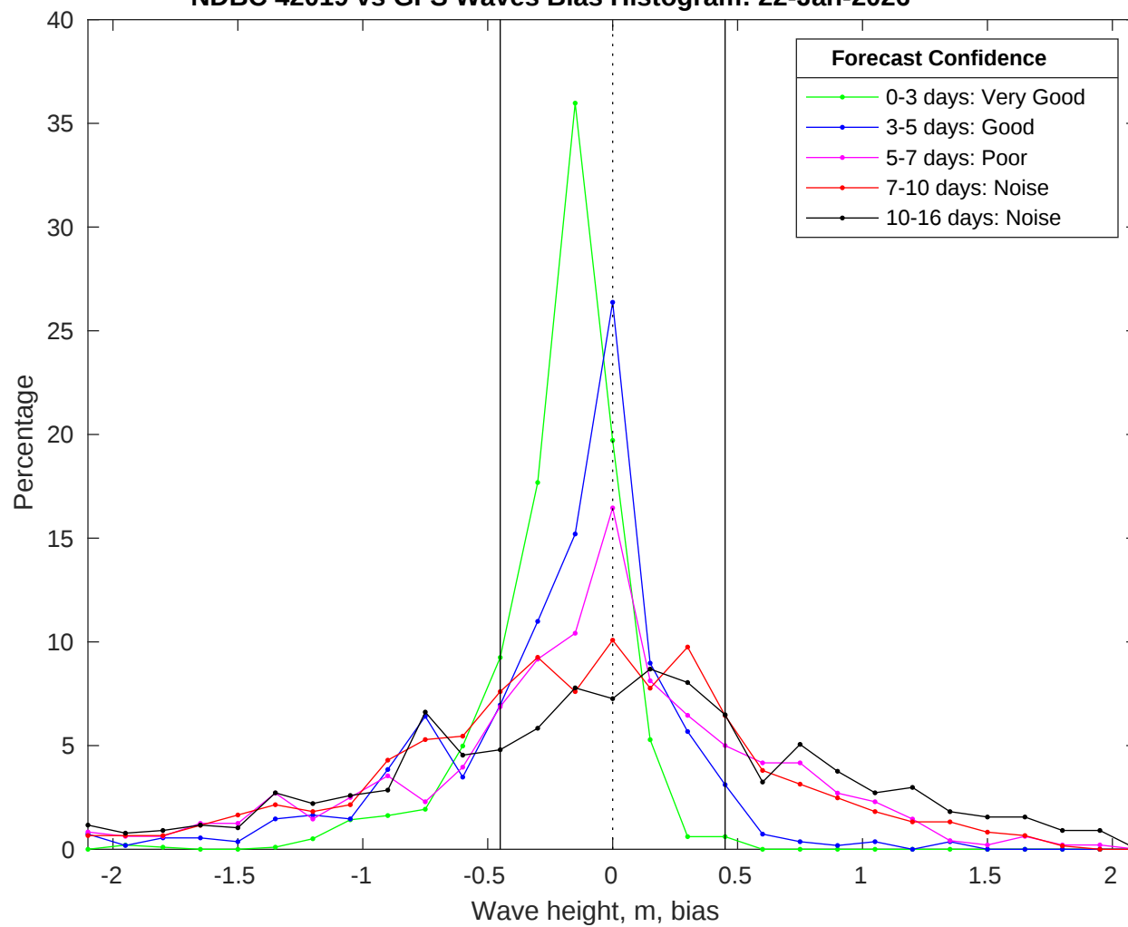
NDBC 42019 vs GFS Waves Bias Histogram: 22-Jan-2026
