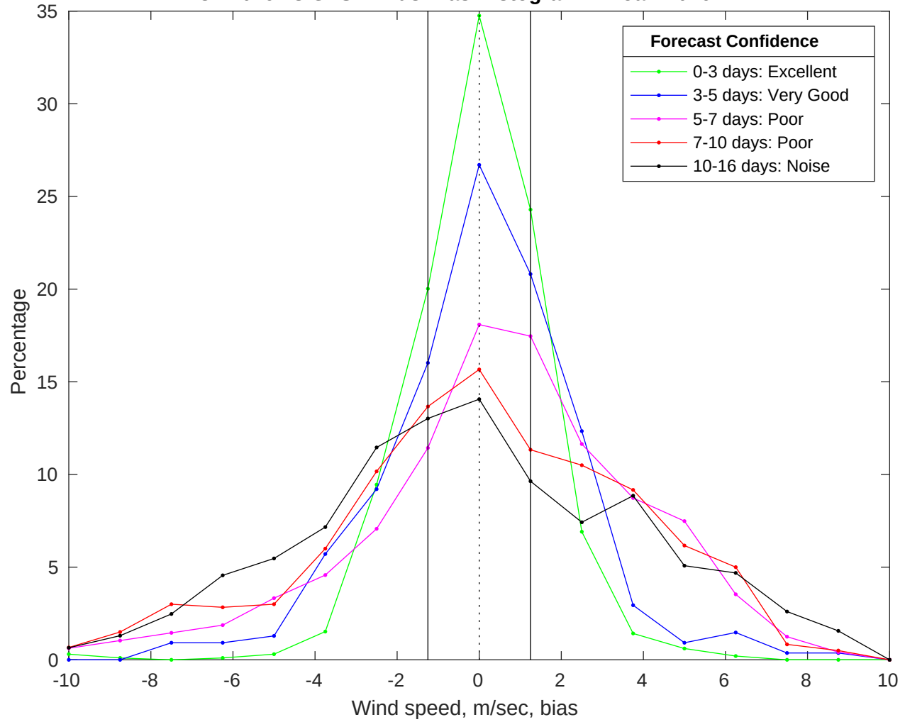
NDBC 42019 vs GFS Winds Bias Histogram: 22-Jan-2026
