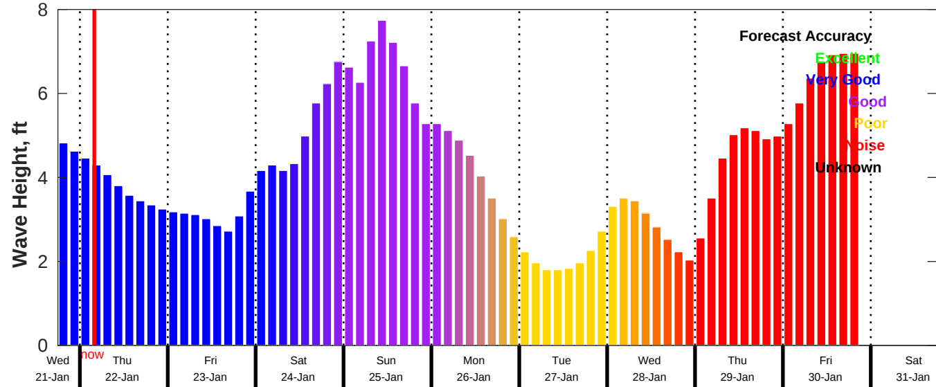
CMEMS Wave Forecast for NDBC 42019 from 21-Jan-2026 18:00:00 to 31-Jan-2026 18:00:00
