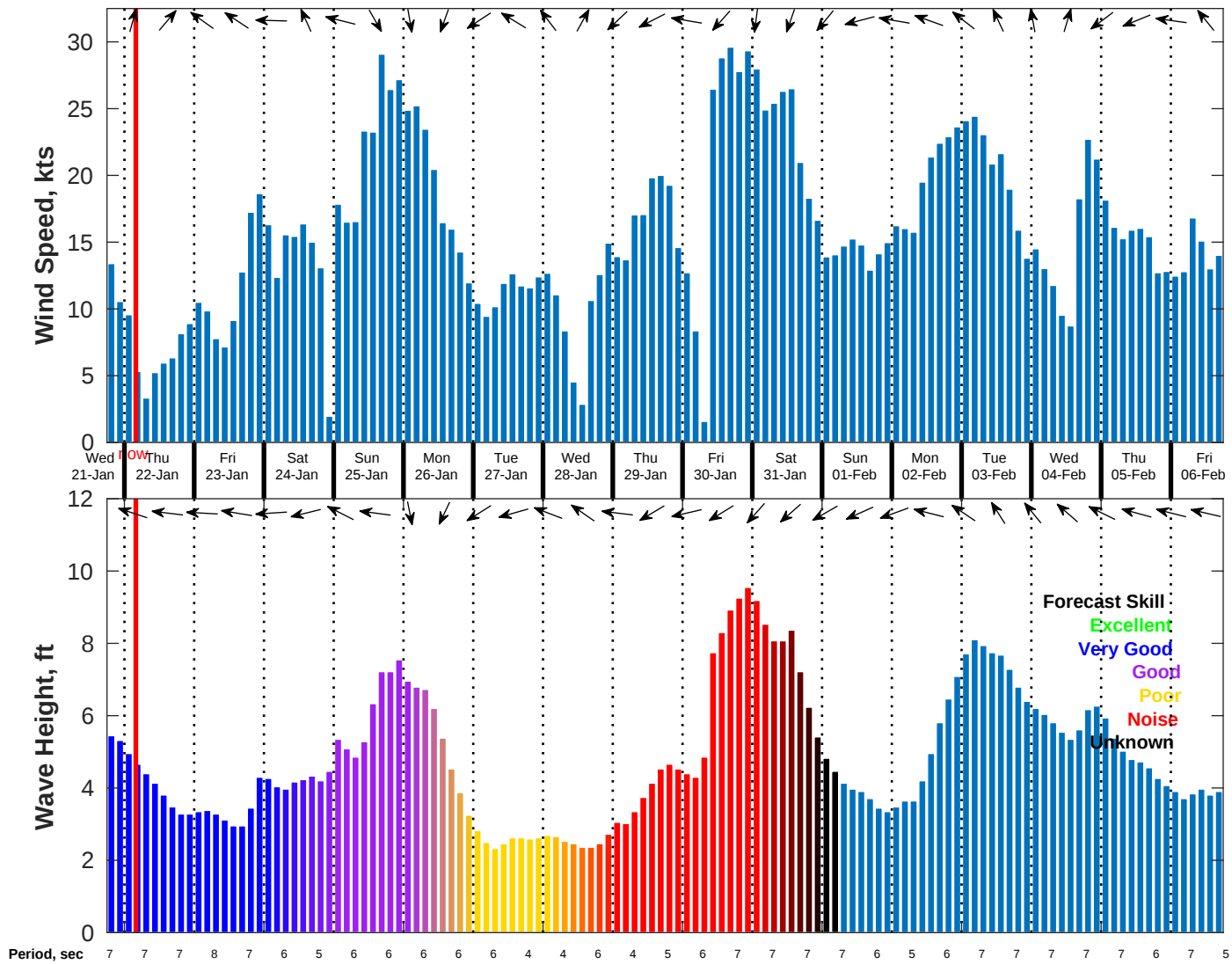
Wind & Wave Forecast for NDBC 42019 from 21-Jan-2026 18:00:00 to 06-Feb-2026 18:00:00
