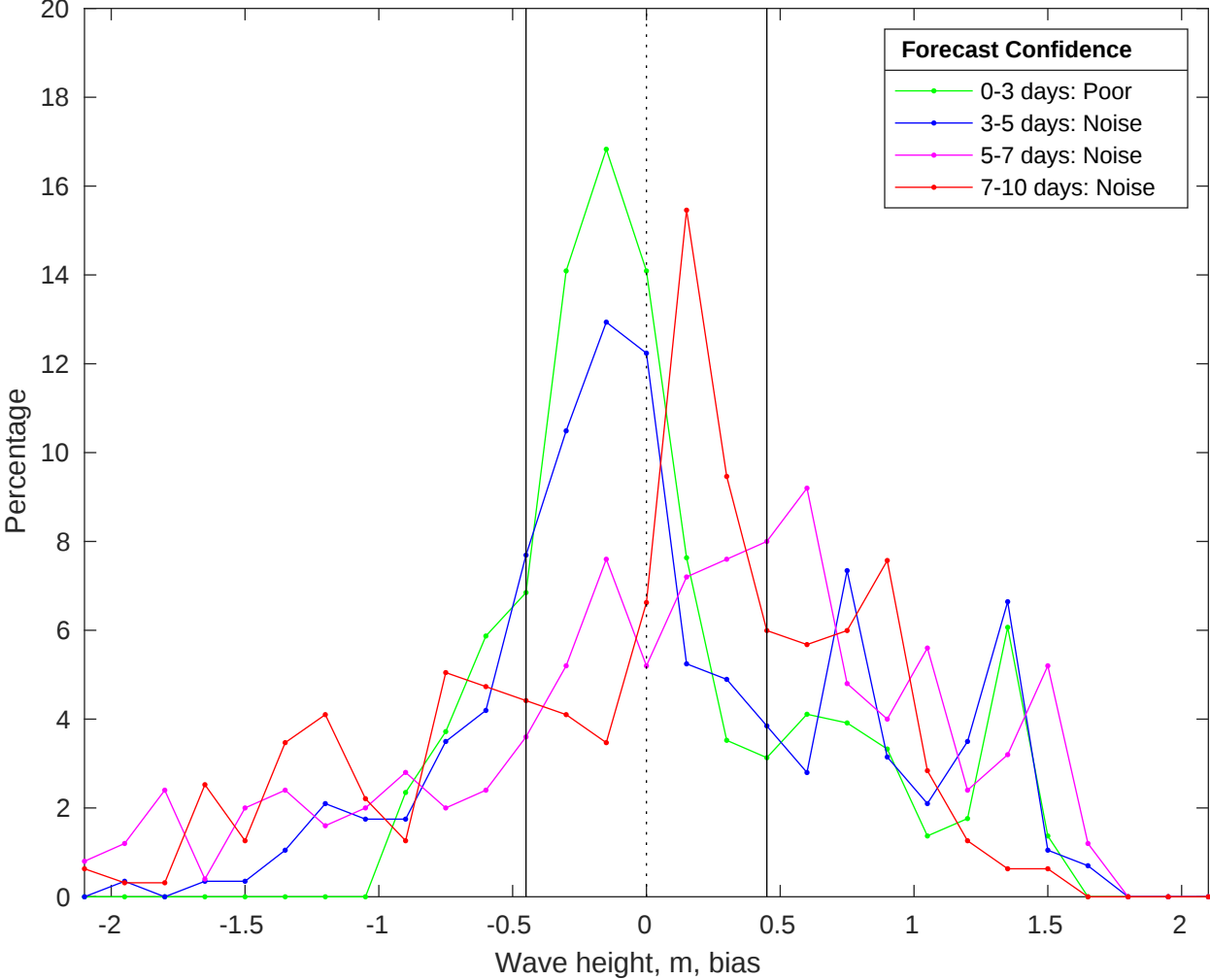
NDBC 42020 vs CMEMS Waves Bias Histogram: 22-Jan-2026
