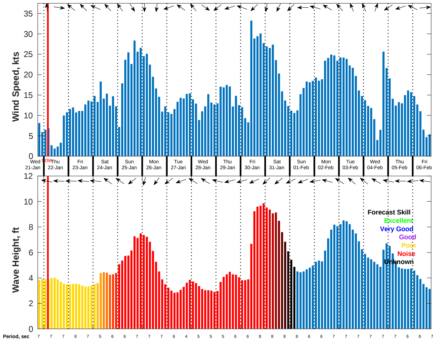
Wind & Wave Forecast for NDBC 42020 from 21-Jan-2026 18:00:00 to 06-Feb-2026 18:00:00
