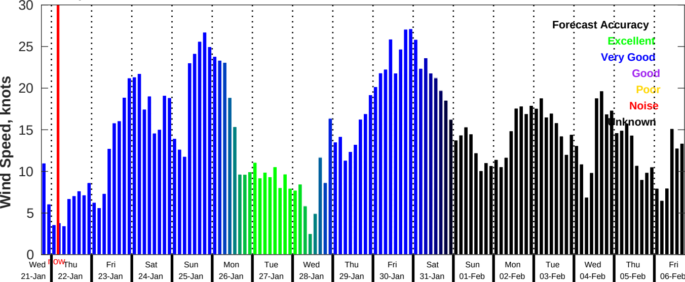
GFS Wind Speed Forecast for NDBC 42035 from 21-Jan-2026 18:00:00 to 06-Feb-2026 18:00:00
