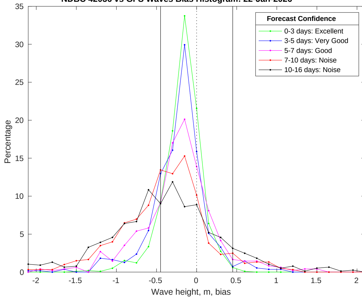
NDBC 42036 vs GFS Waves Bias Histogram: 22-Jan-2026
