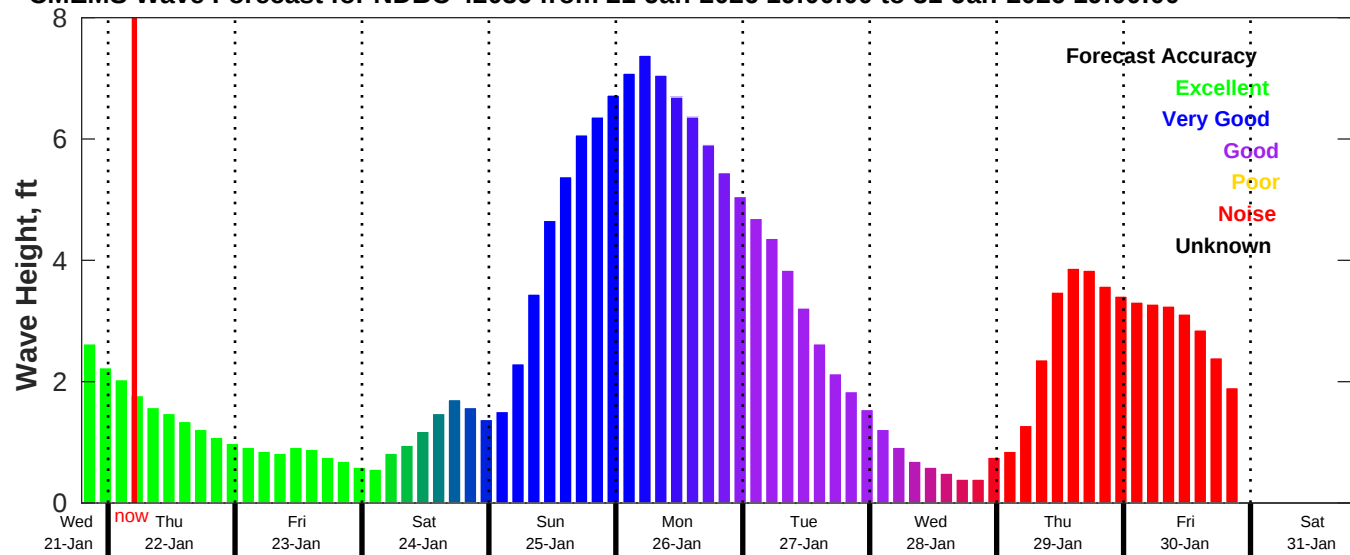
CMEMS Wave Forecast for NDBC 42036 from 21-Jan-2026 19:00:00 to 31-Jan-2026 19:00:00
