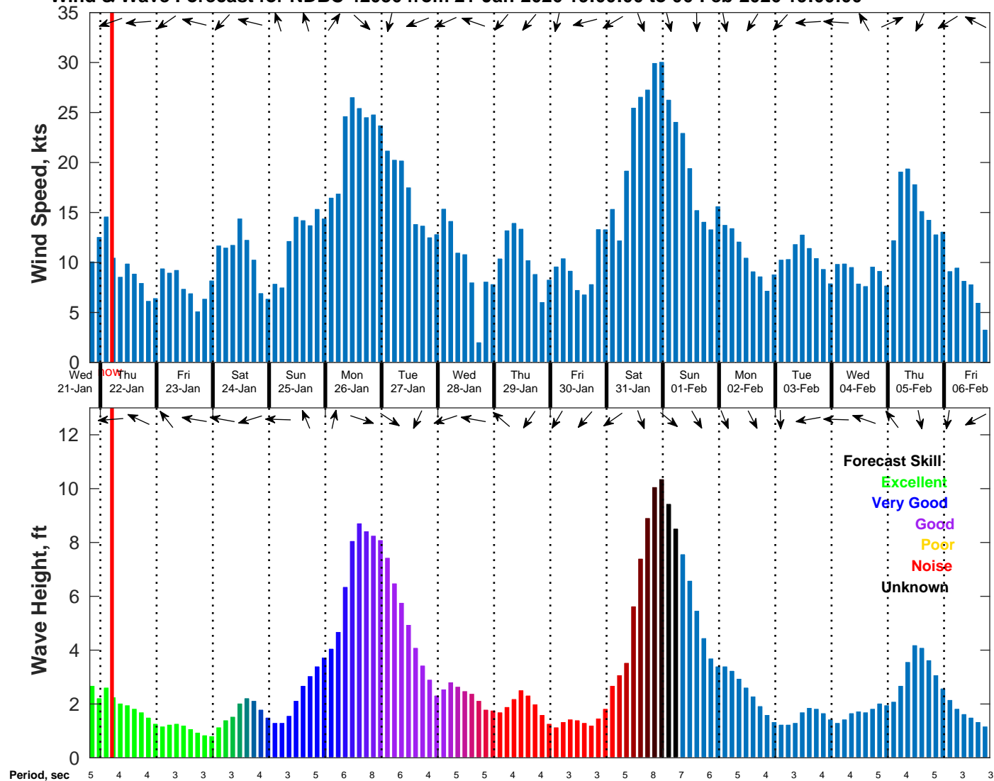
Wind & Wave Forecast for NDBC 42036 from 21-Jan-2026 19:00:00 to 06-Feb-2026 19:00:00
