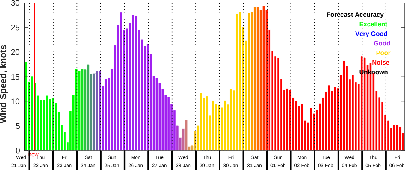
GFS Wind Speed Forecast for NDBC 42040 from 21-Jan-2026 19:00:00 to 06-Feb-2026 19:00:00
