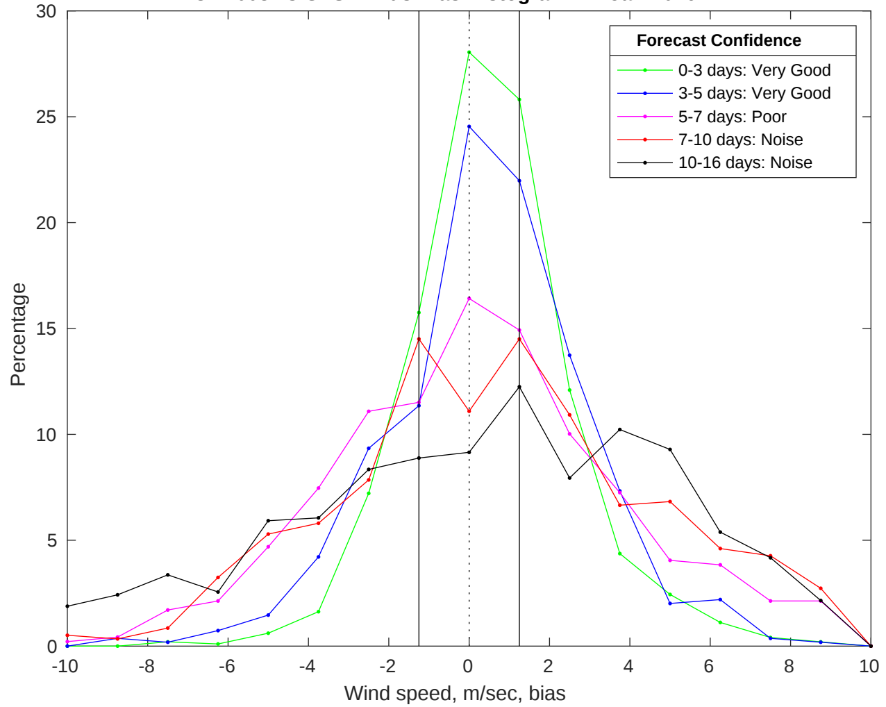
NDBC 44008 vs GFS Winds Bias Histogram: 22-Jan-2026
