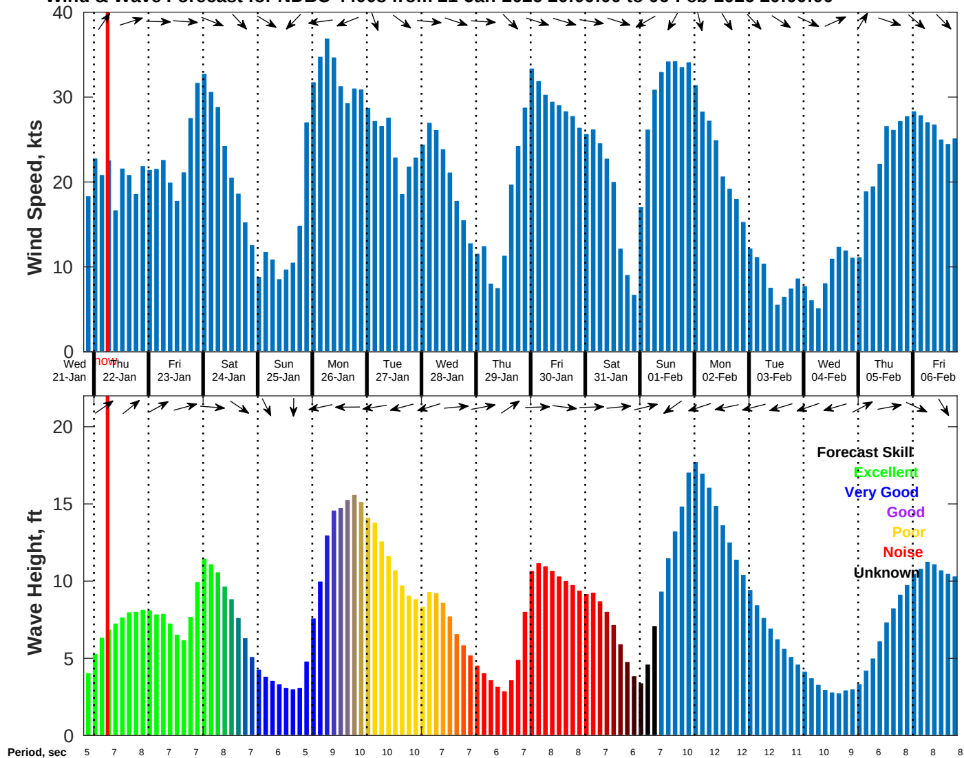
Wind & Wave Forecast for NDBC 44008 from 21-Jan-2026 20:00:00 to 06-Feb-2026 20:00:00
