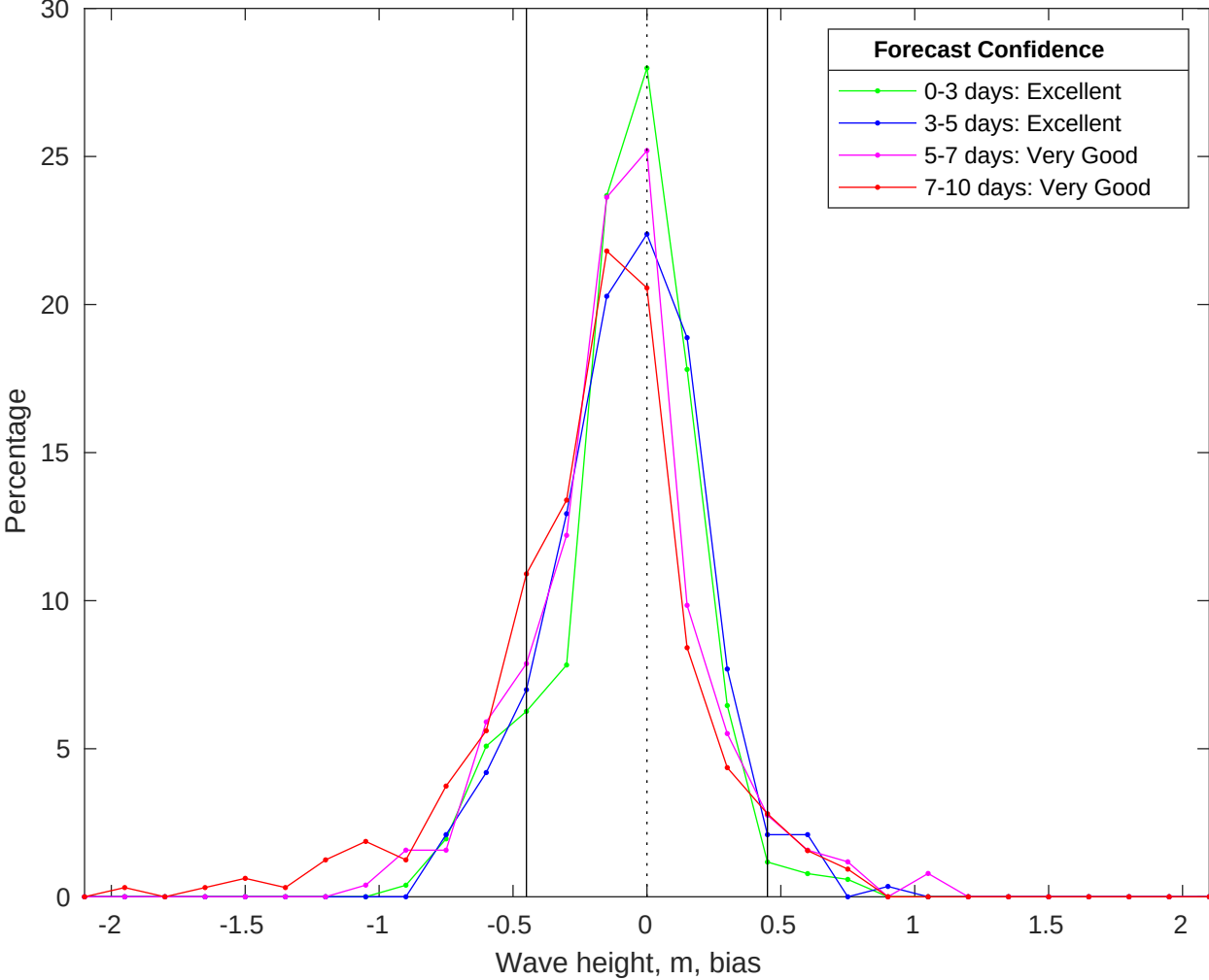
NDBC 46011 vs CMEMS Waves Bias Histogram: 22-Jan-2026
