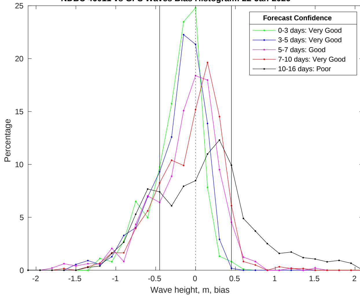
NDBC 46011 vs GFS Waves Bias Histogram: 22-Jan-2026
