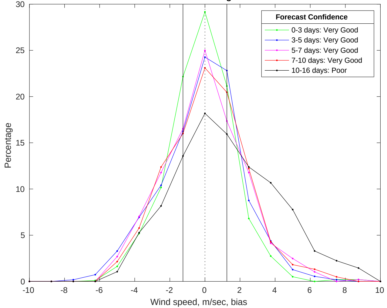
NDBC 46011 vs GFS Winds Bias Histogram: 22-Jan-2026
