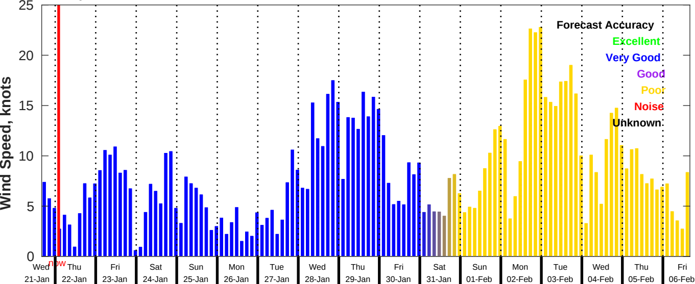
GFS Wind Speed Forecast for NDBC 46011 from 21-Jan-2026 16:00:00 to 06-Feb-2026 16:00:00
