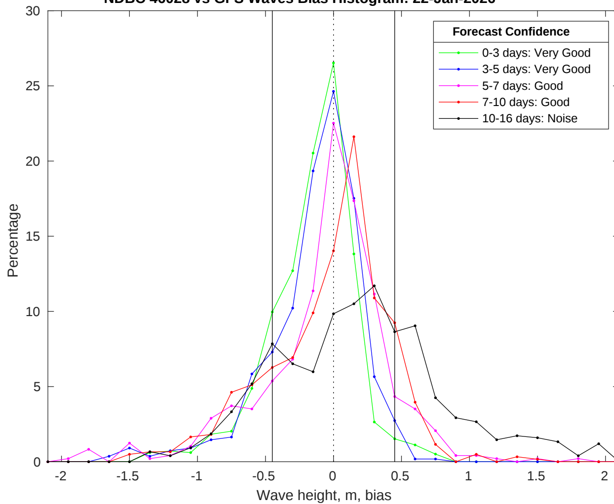
NDBC 46028 vs GFS Waves Bias Histogram: 22-Jan-2026
