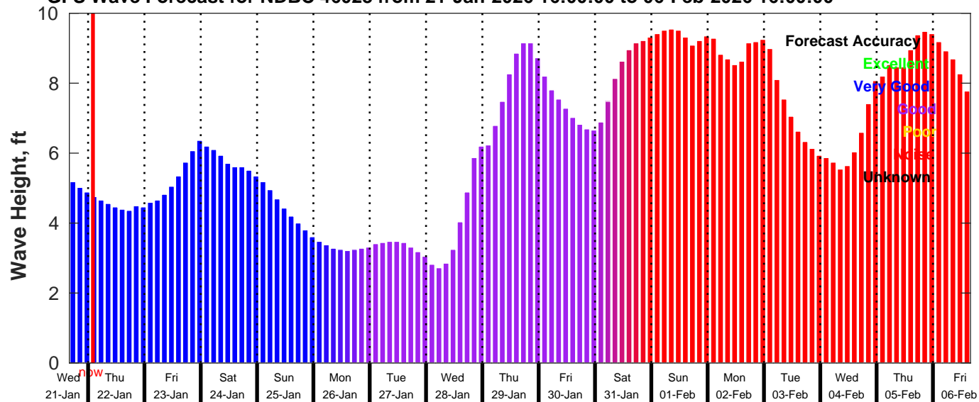
GFS Wave Forecast for NDBC 46028 from 21-Jan-2026 16:00:00 to 06-Feb-2026 16:00:00
