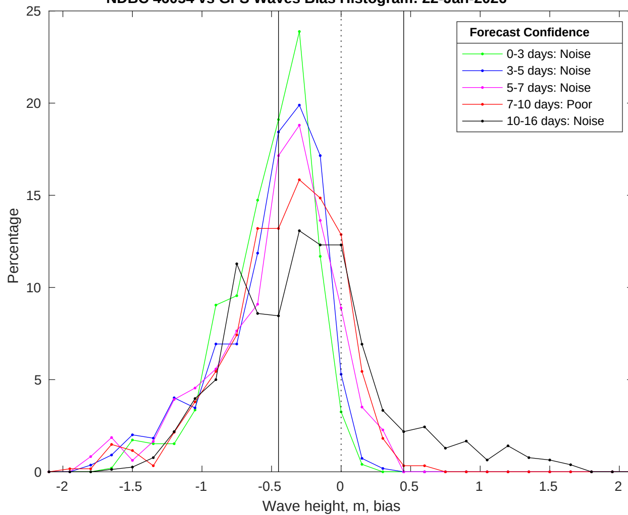
NDBC 46054 vs GFS Waves Bias Histogram: 22-Jan-2026
