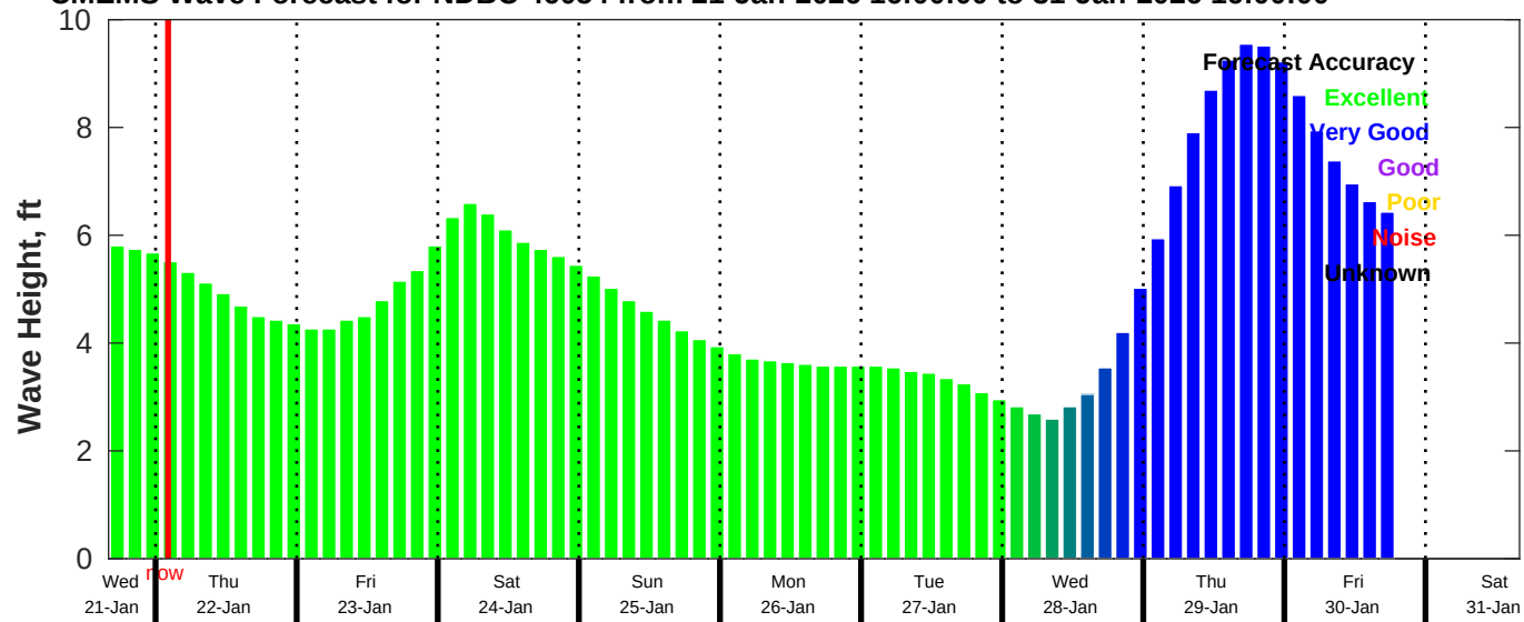
CMEMS Wave Forecast for NDBC 46054 from 21-Jan-2026 16:00:00 to 31-Jan-2026 16:00:00
