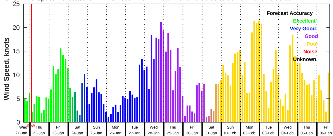
GFS Wind Speed Forecast for NDBC 46054 from 21-Jan-2026 16:00:00 to 06-Feb-2026 16:00:00
