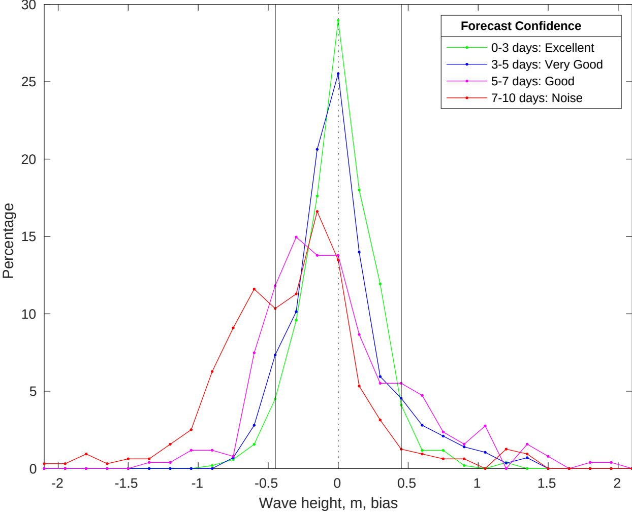
NDBC 46059 vs CMEMS Waves Bias Histogram: 22-Jan-2026
