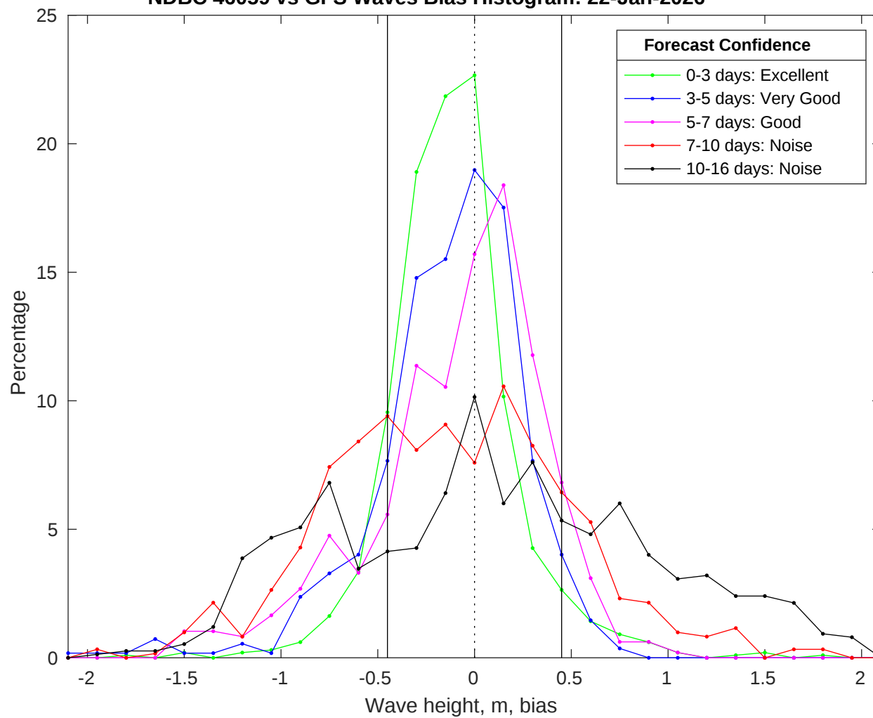
NDBC 46059 vs GFS Waves Bias Histogram: 22-Jan-2026
