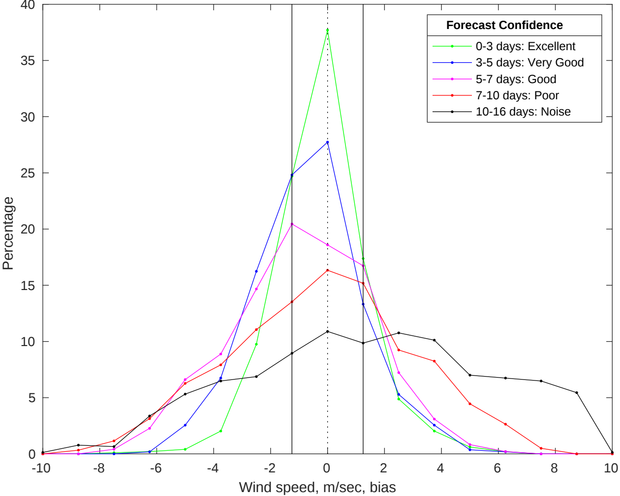
NDBC 46059 vs GFS Winds Bias Histogram: 22-Jan-2026
