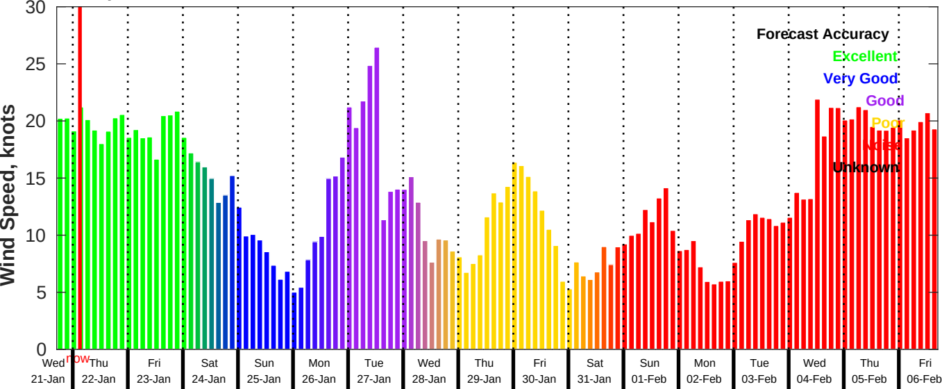
GFS Wind Speed Forecast for NDBC 46059 from 21-Jan-2026 17:00:00 to 06-Feb-2026 17:00:00
