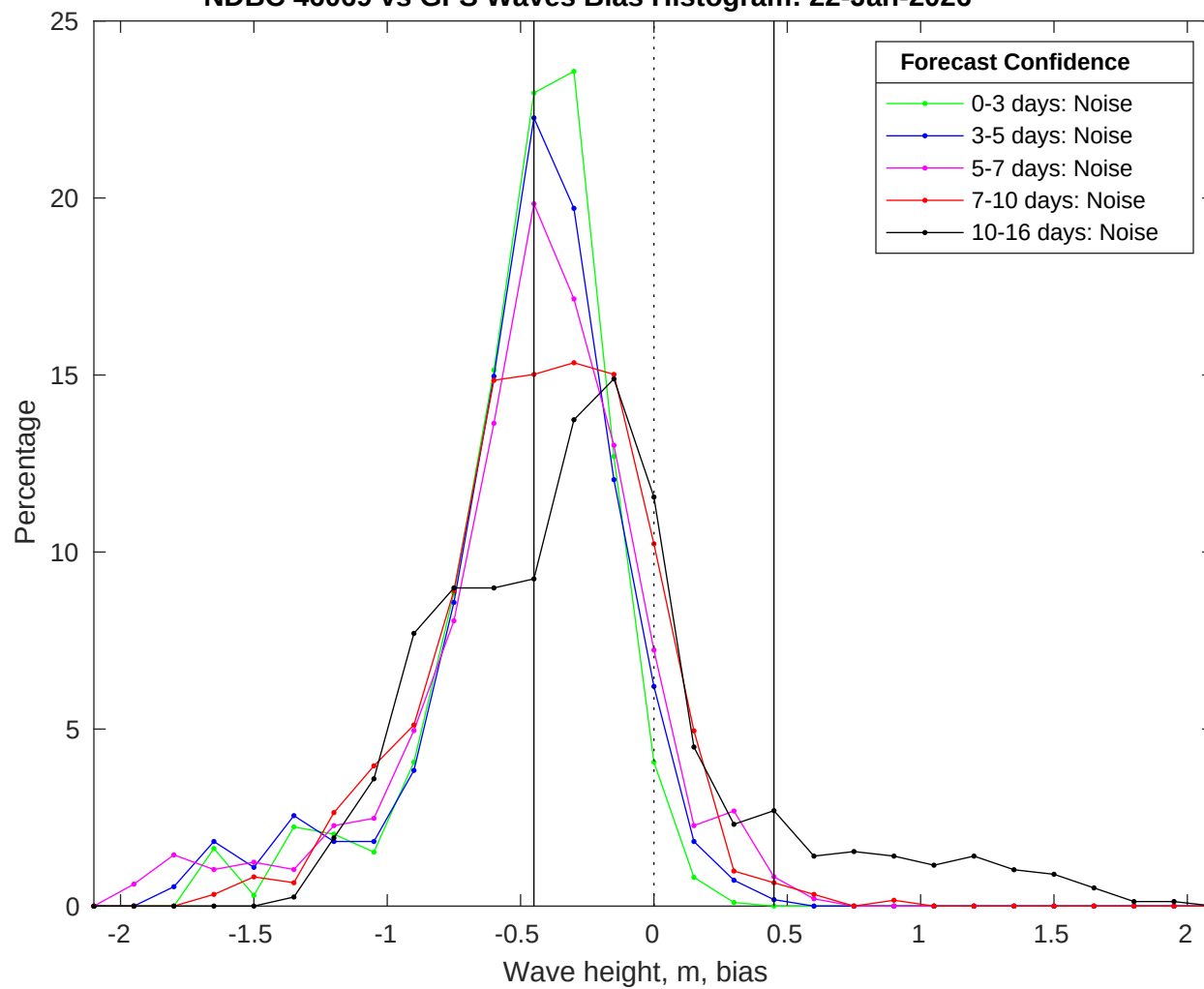
NDBC 46069 vs GFS Waves Bias Histogram: 22-Jan-2026
