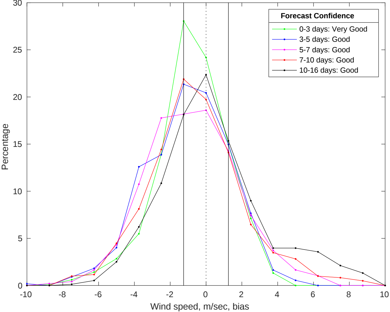
NDBC 46069 vs GFS Winds Bias Histogram: 22-Jan-2026
