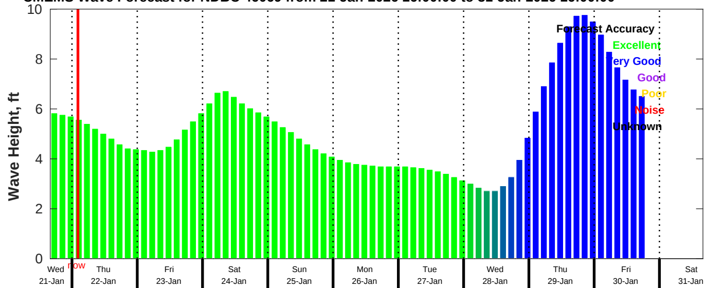
CMEMS Wave Forecast for NDBC 46069 from 21-Jan-2026 16:00:00 to 31-Jan-2026 16:00:00
