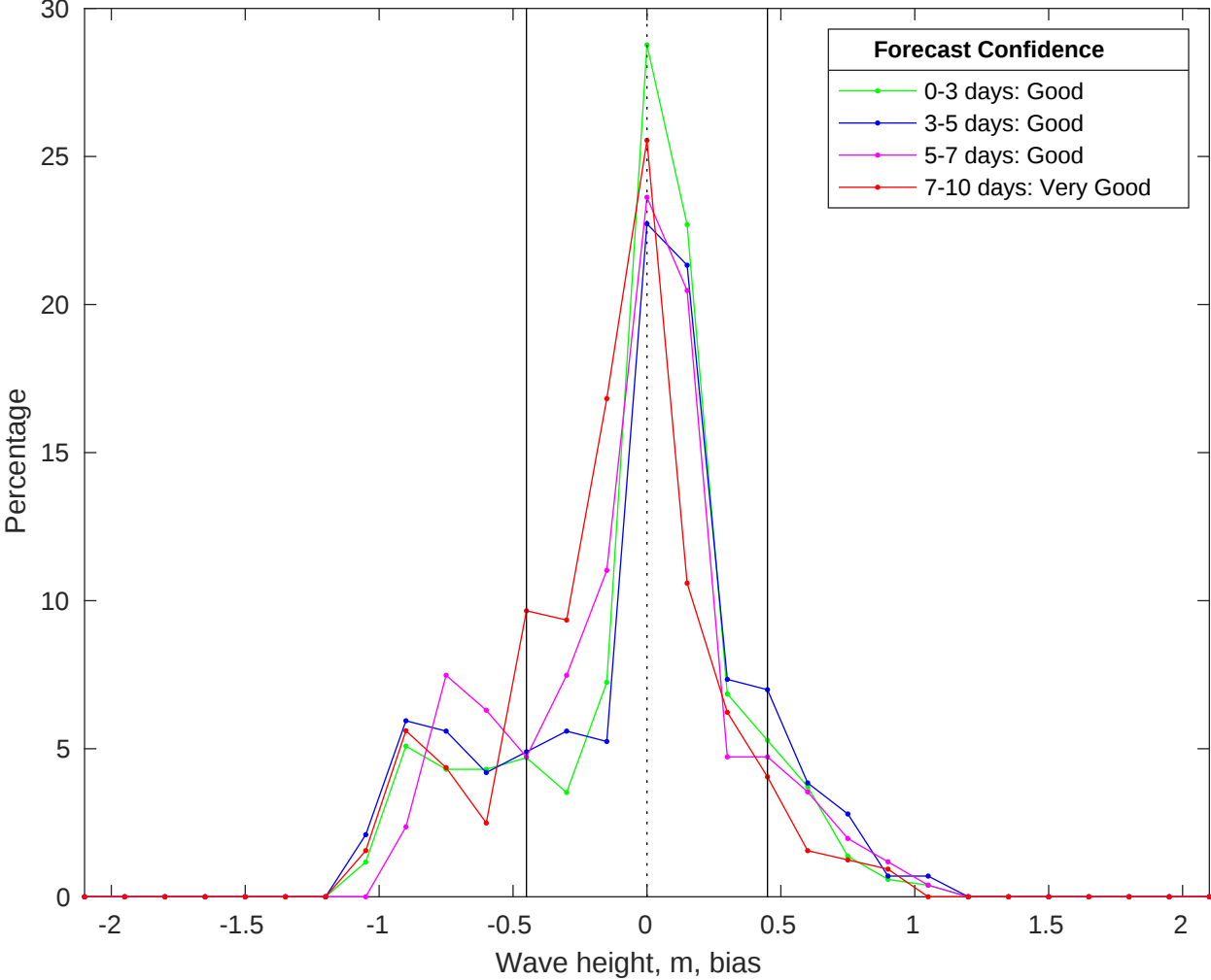
NDBC 46215 vs CMEMS Waves Bias Histogram: 22-Jan-2026
