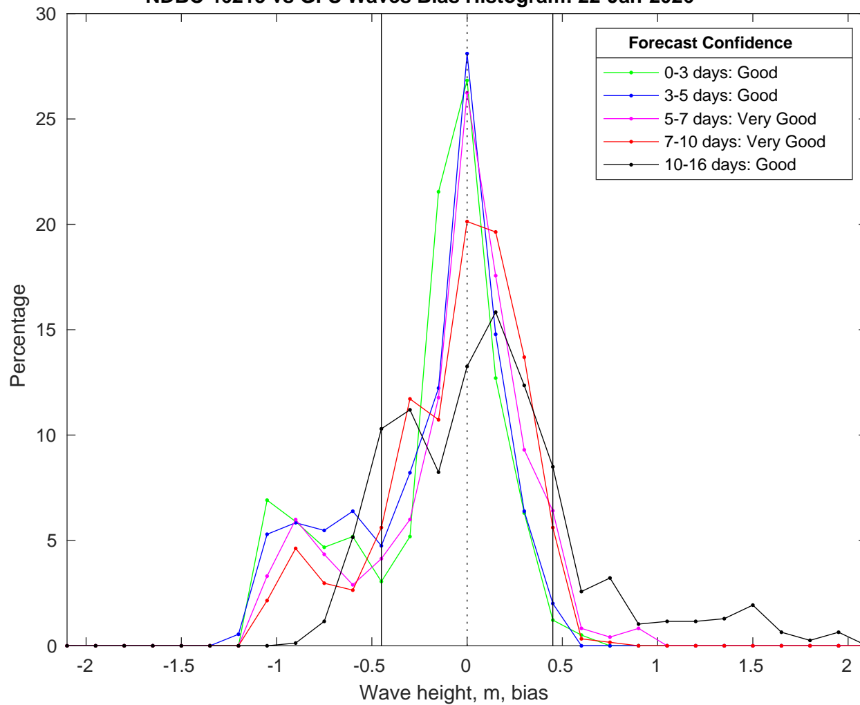
NDBC 46215 vs GFS Waves Bias Histogram: 22-Jan-2026
