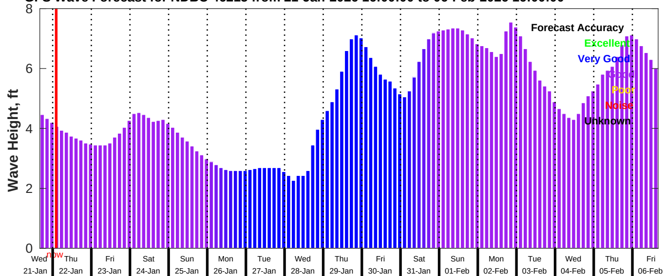
GFS Wave Forecast for NDBC 46215 from 21-Jan-2026 16:00:00 to 06-Feb-2026 16:00:00
