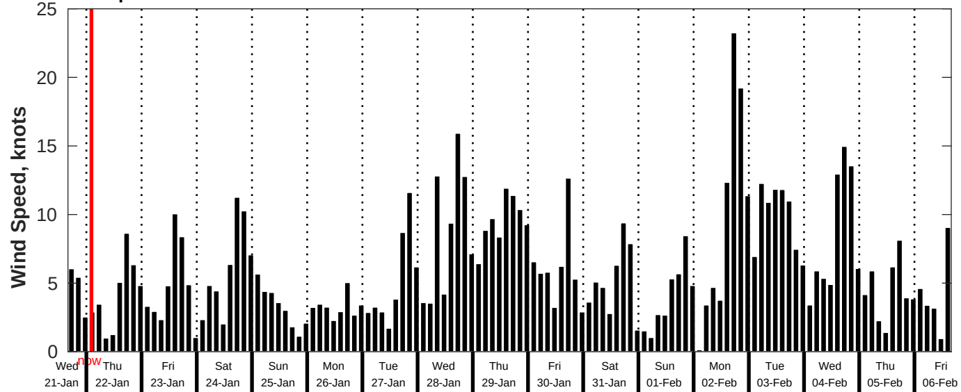
GFS Wind Speed Forecast for NDBC 46215 from 21-Jan-2026 16:00:00 to 06-Feb-2026 16:00:00
