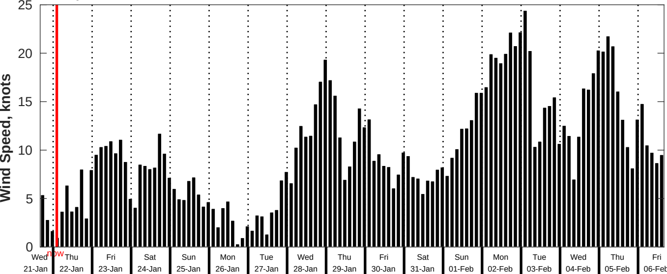
GFS Wind Speed Forecast for NDBC 46259 from 21-Jan-2026 16:00:00 to 06-Feb-2026 16:00:00
