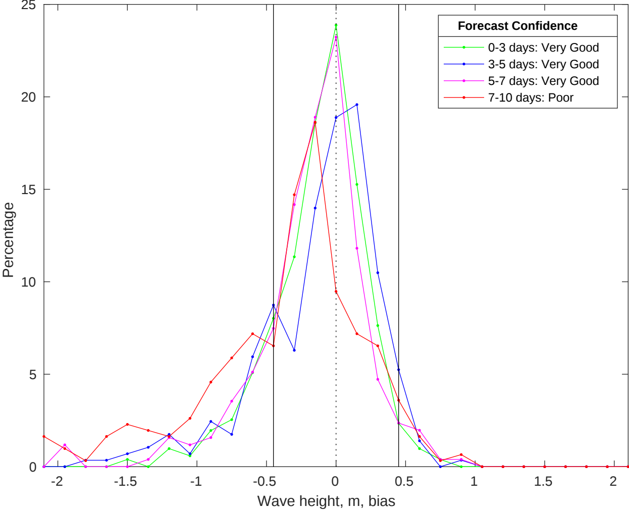
NDBC 51000 vs CMEMS Waves Bias Histogram: 22-Jan-2026
