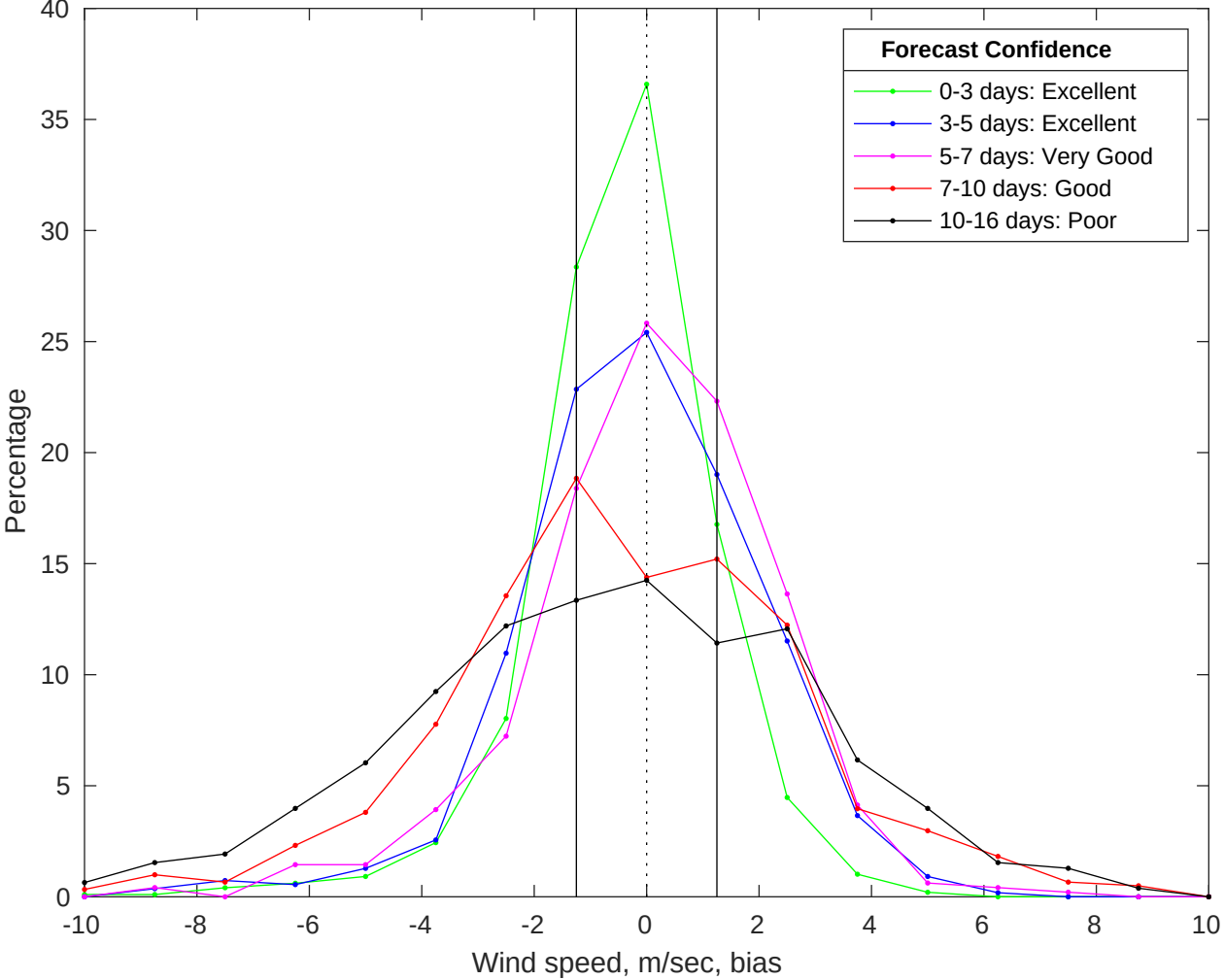
NDBC 51000 vs GFS Winds Bias Histogram: 22-Jan-2026
