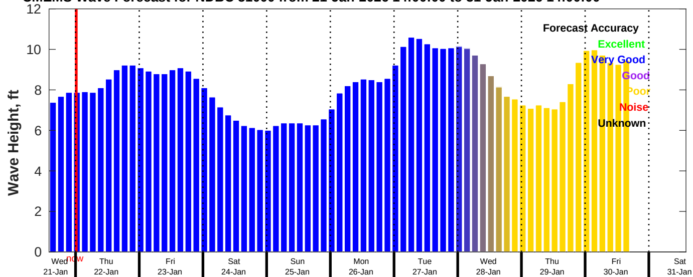
CMEMS Wave Forecast for NDBC 51000 from 21-Jan-2026 14:00:00 to 31-Jan-2026 14:00:00
