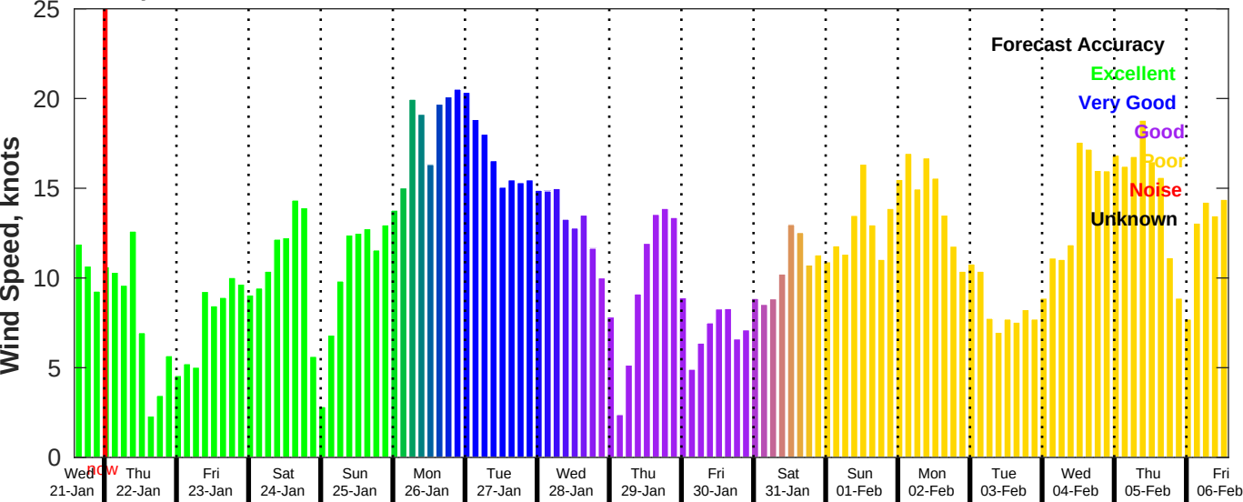
GFS Wind Speed Forecast for NDBC 51000 from 21-Jan-2026 14:00:00 to 06-Feb-2026 14:00:00
