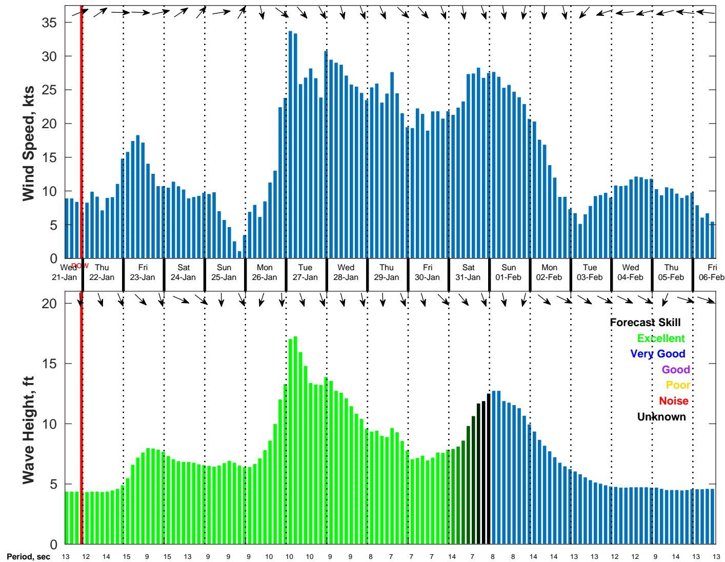
Wind & Wave Forecast for NDBC 51209 from 21-Jan-2026 13:00:00 to 06-Feb-2026 13:00:00
