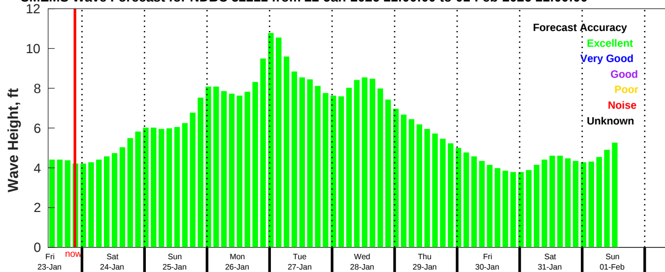
CMEMS Wave Forecast for NDBC 52211 from 22-Jan-2026 11:00:00 to 01-Feb-2026 11:00:00
