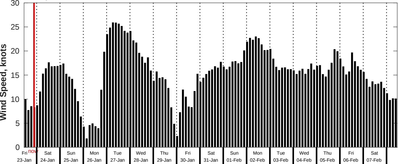
GFS Wind Speed Forecast for NDBC 52211 from 22-Jan-2026 11:00:00 to 07-Feb-2026 11:00:00
