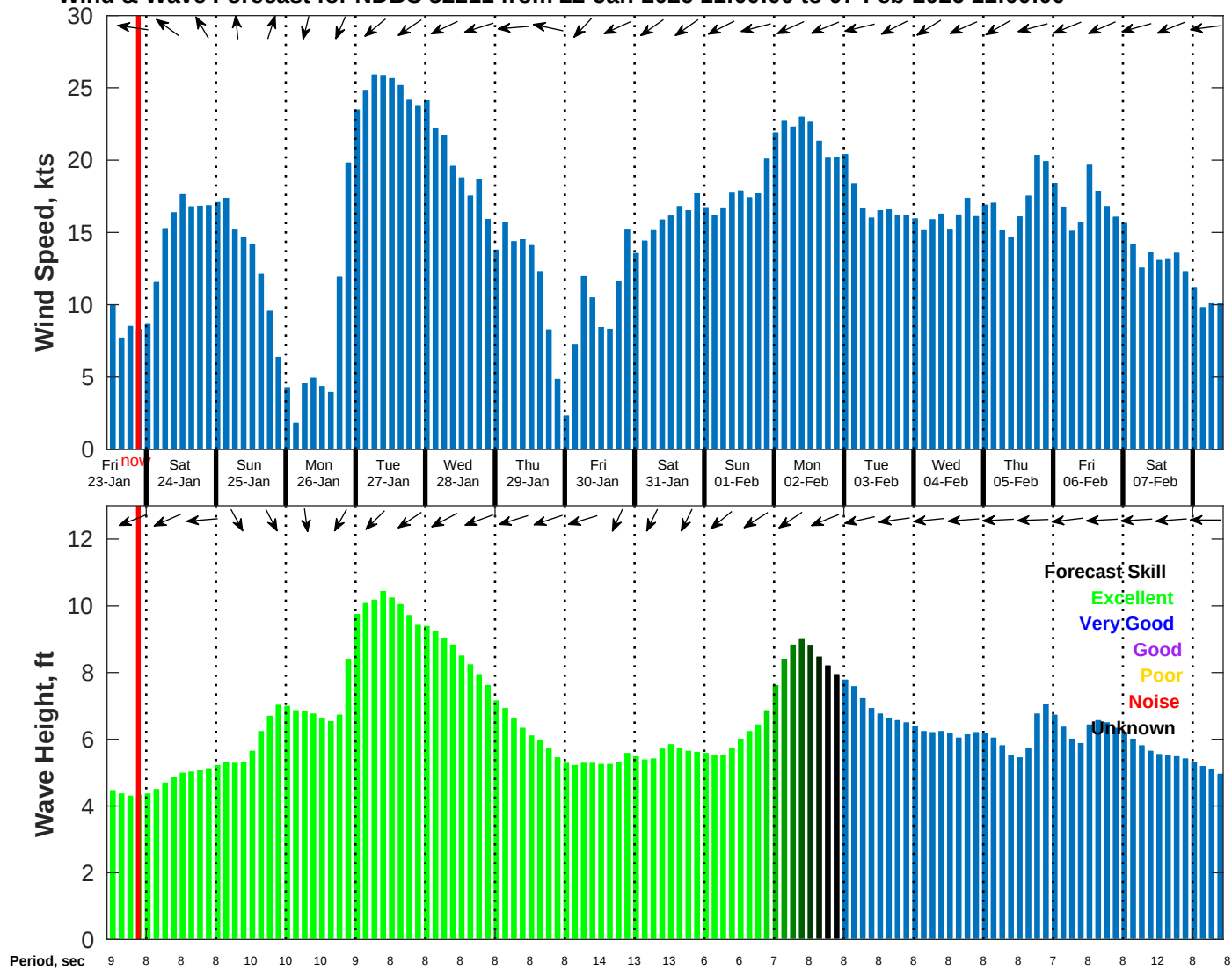
Wind & Wave Forecast for NDBC 52211 from 22-Jan-2026 11:00:00 to 07-Feb-2026 11:00:00
