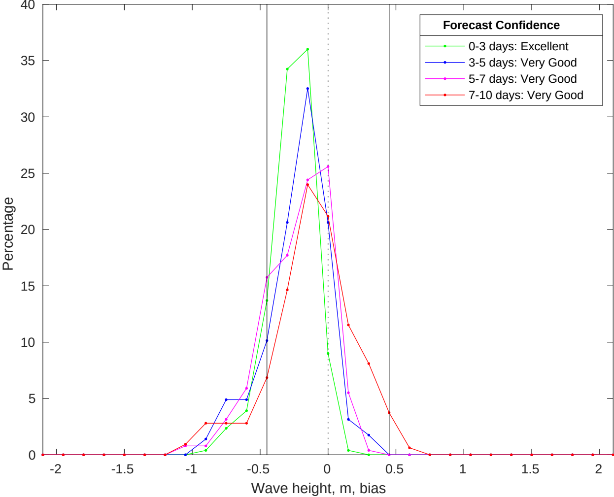
NDBC 52213 vs CMEMS Waves Bias Histogram: 22-Jan-2026
