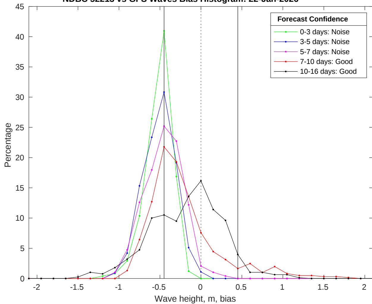
NDBC 52213 vs GFS Waves Bias Histogram: 22-Jan-2026
