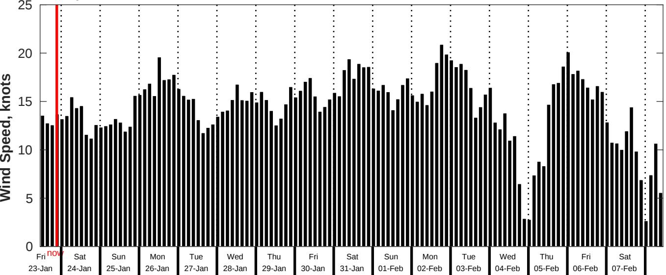
GFS Wind Speed Forecast for NDBC 52213 from 22-Jan-2026 11:00:00 to 07-Feb-2026 11:00:00
