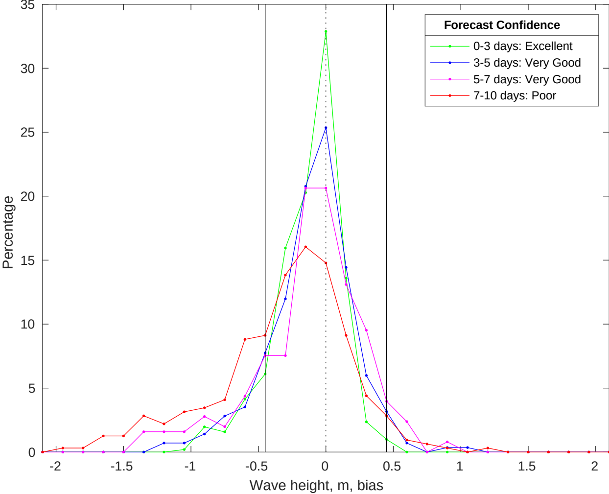
NDBC 41004 vs CMEMS Waves Bias Histogram: 23-Jan-2026
