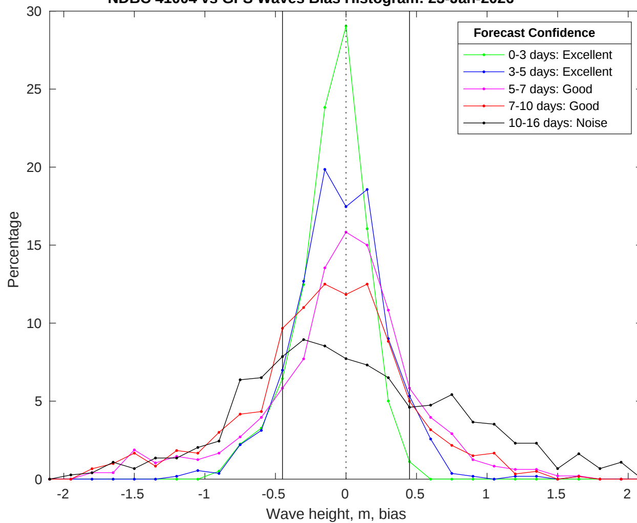
NDBC 41004 vs GFS Waves Bias Histogram: 23-Jan-2026
